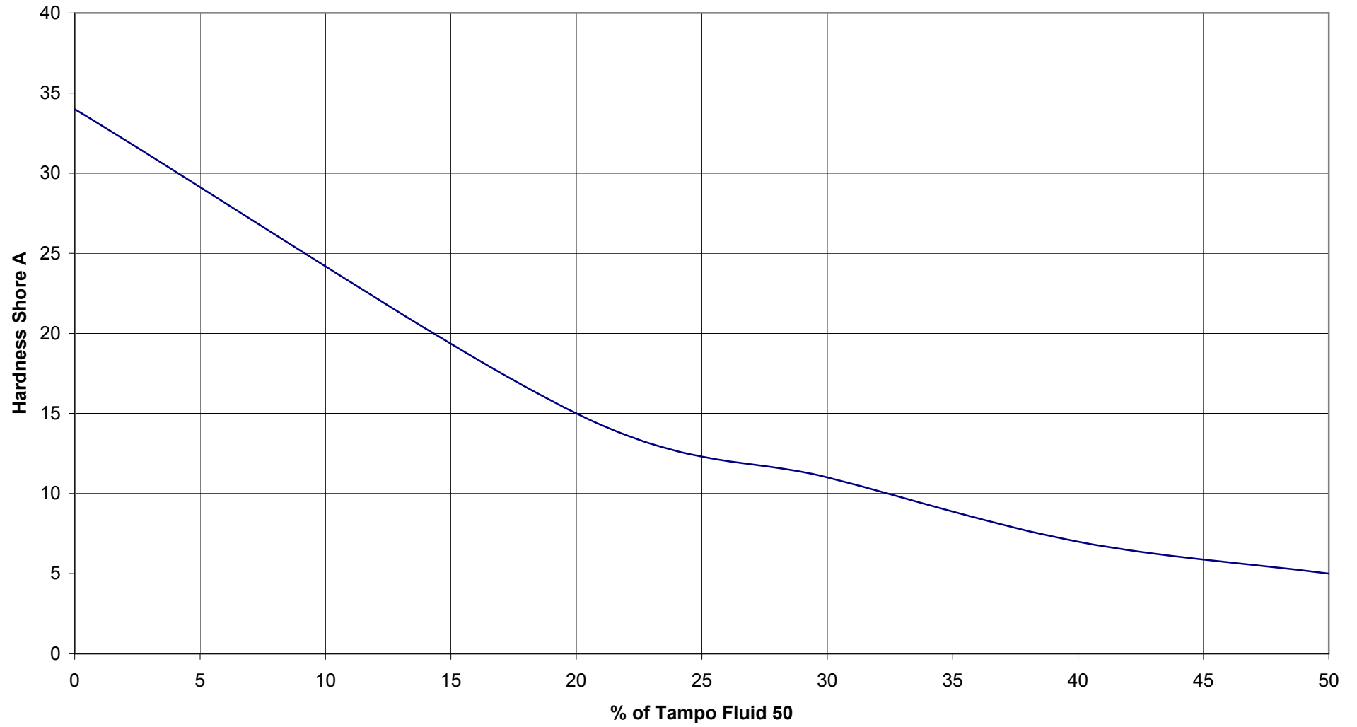
MM230 Dilution With Tampo 50 Fluid Shore A 7 Days
