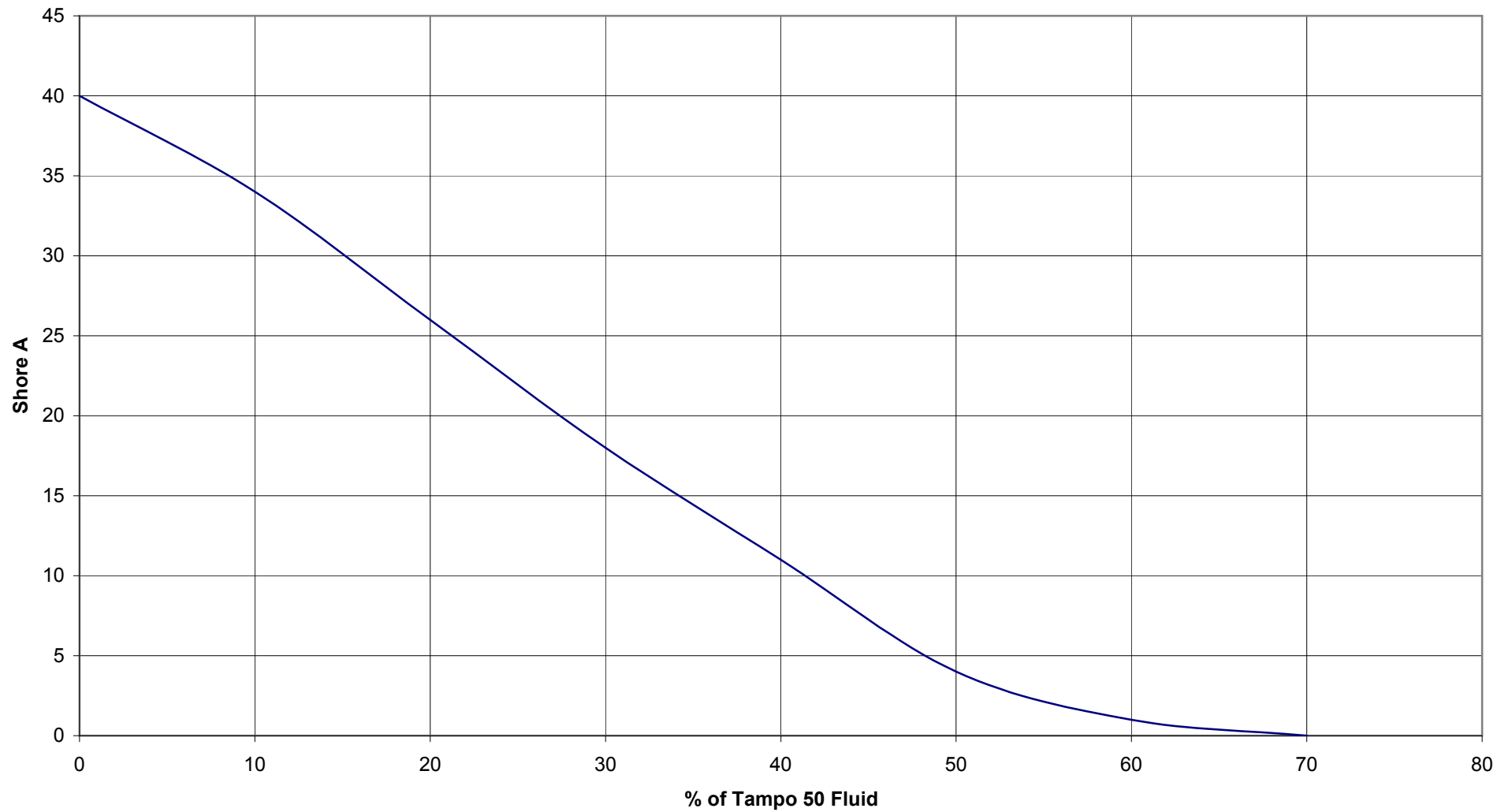
MM242 Tampo 50 Fluid Dilutions Shore A After 7 Days
